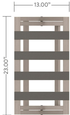
plan
